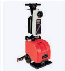
Ocelot Plus 400 39-094 The Ocelot Plus features all the capabilities of the Ocelot 400, but with the addition of vacuumation for wet pick up.
